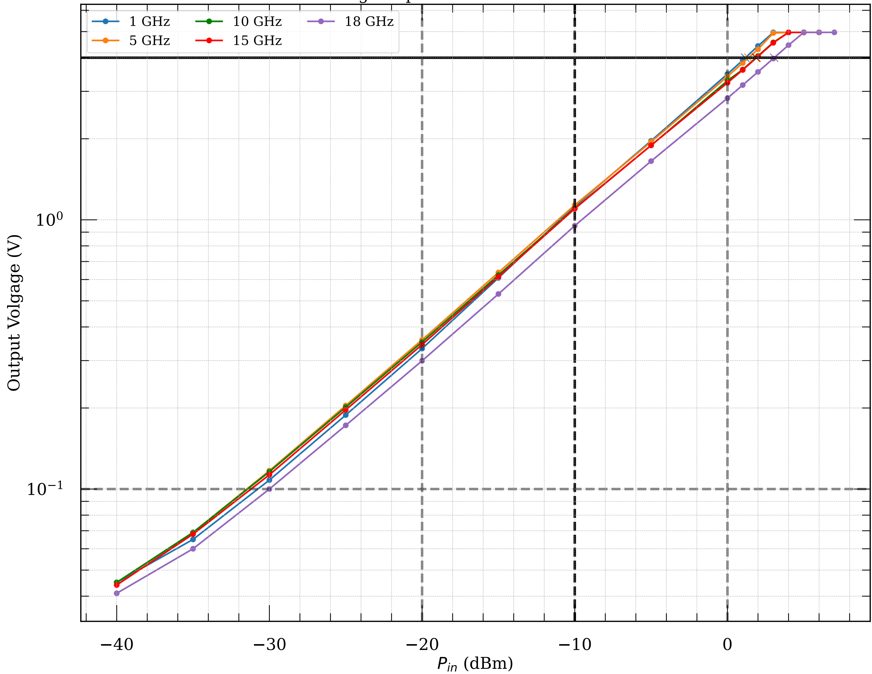
Measured voltage-to-power curve of detector module094v2
